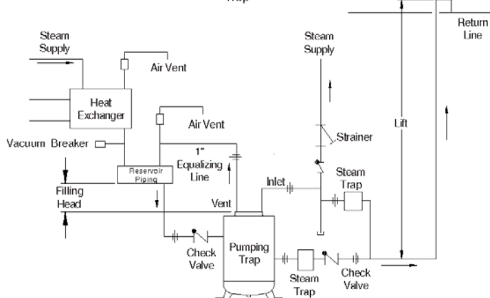
FIGURE 8 : Drainage from a heat exchanger in a closed-loop system where the supply pressure may be higher or lower than the back pressure. If the heat exchanger pressure exceeds the back pressure the pumping trap will be idle and the steam trap will prevent the steam from "blowing through" into the return line. Motive force of steam is depicted.
